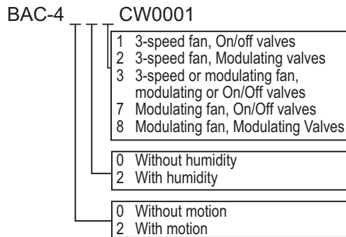
Illustration 1—Fan Coil Unit models
