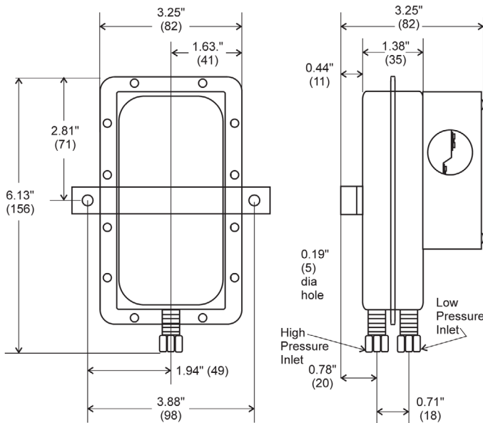
Nominal Dimensions in Inches (Millimeters)
