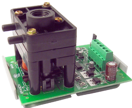
XEC-3001/3004 E to P transducer
