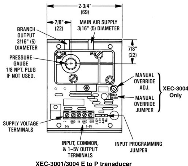
XEC-3001/3004 E to P transducer
