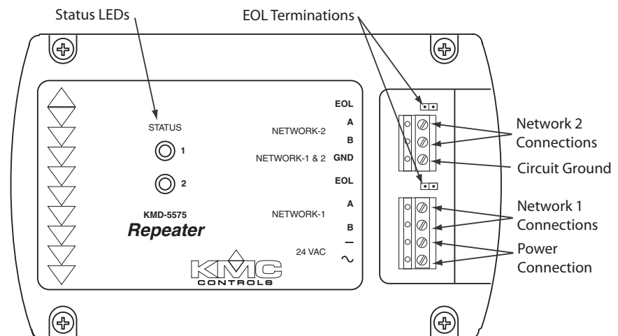
Illustration 1 – Components
