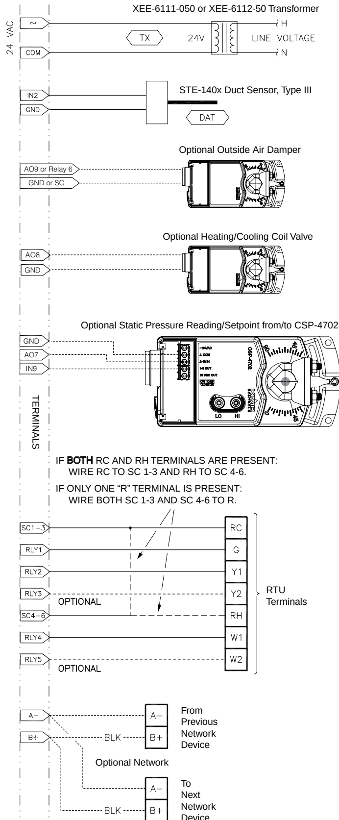
Illustration 4—HPU Application Connections
