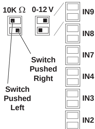
Illustration 8—EOL/Pull-Up Switch Positions
