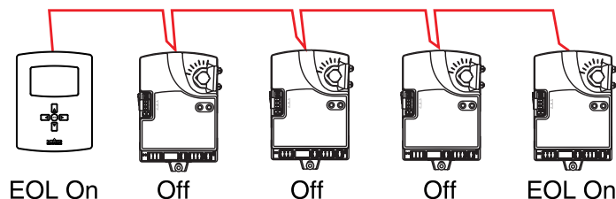
Illustration 7—MS/TP Network End-Of-Line Termination
