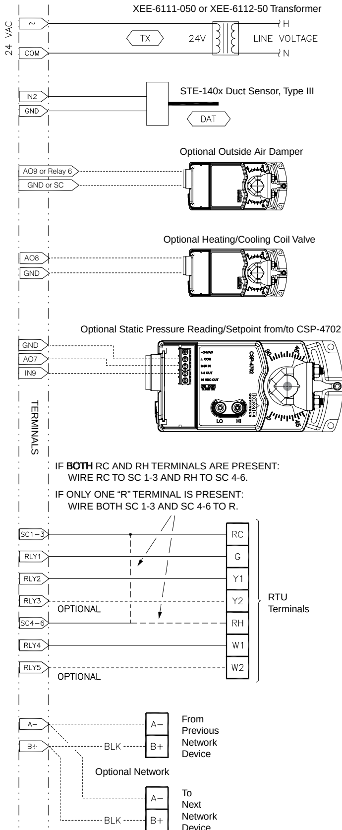
Illustration 3—RTU Application Connections
