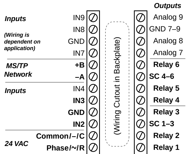
Illustration 5—Terminals and Connections
