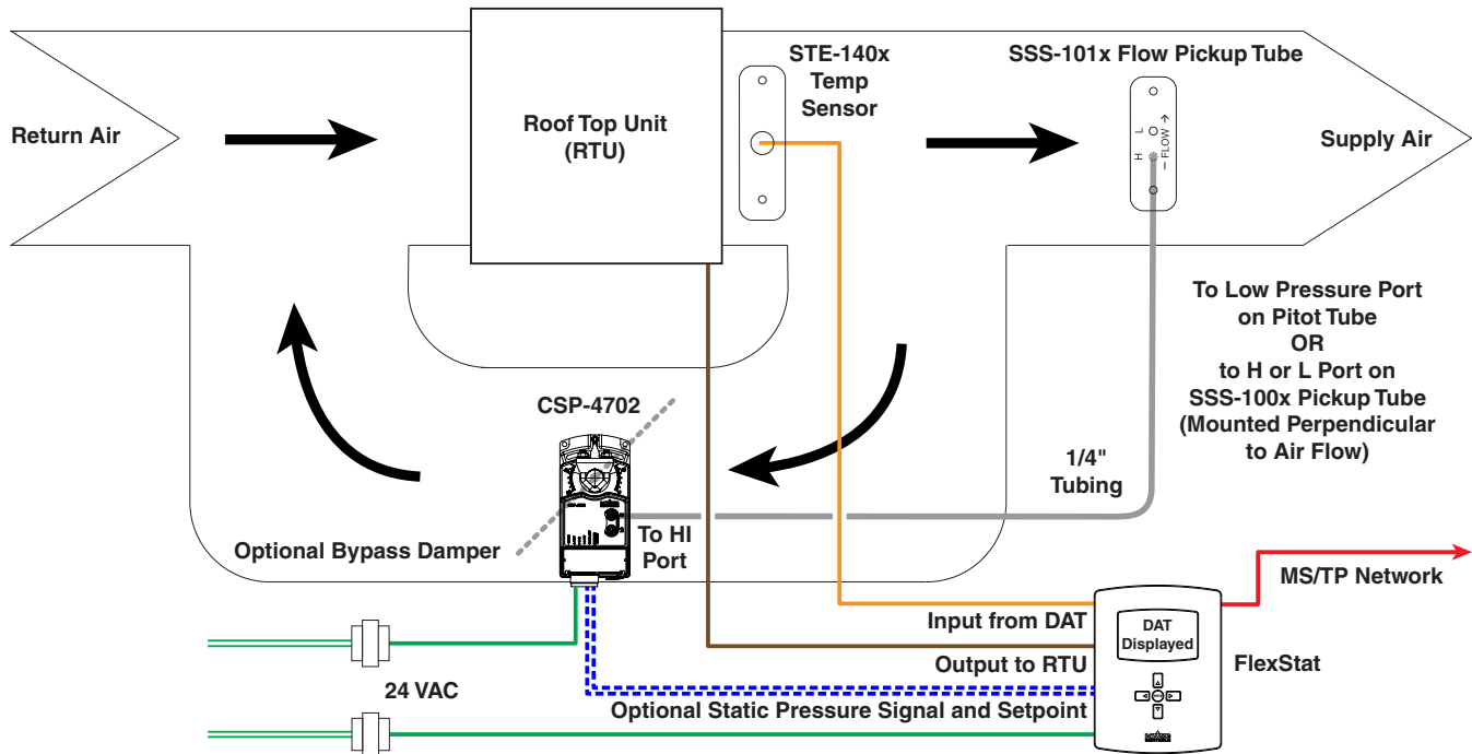
RTU Controller—MAC 20, Device Instance 1000000
