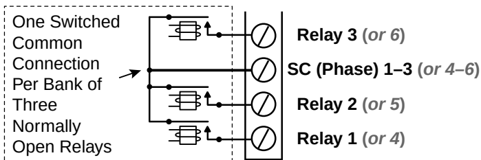
Illustration 6—Switched (Relay) Common and Relays
