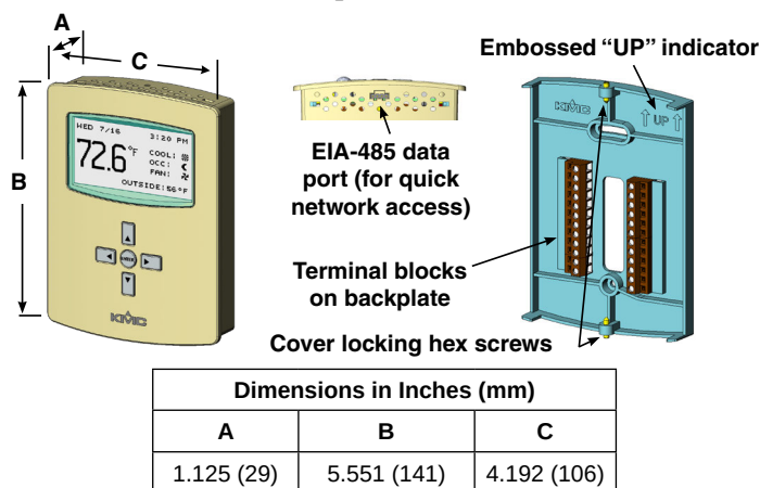
Illustration 1—Dimensions and Installation
