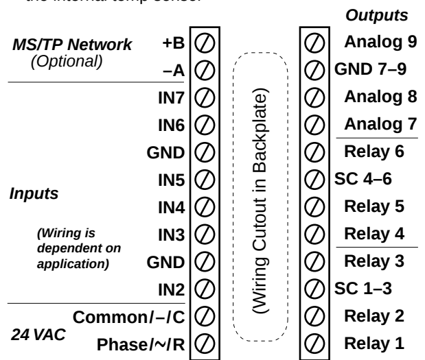
Illustration 5—BAC-19xx63-ZEC Terminals and Connections
