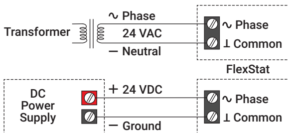
Illustration 12—Power Terminals
