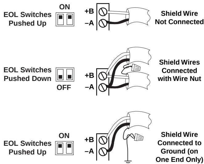
Illustration 10—MS/TP Connections and EOL (MS/TP Models)
