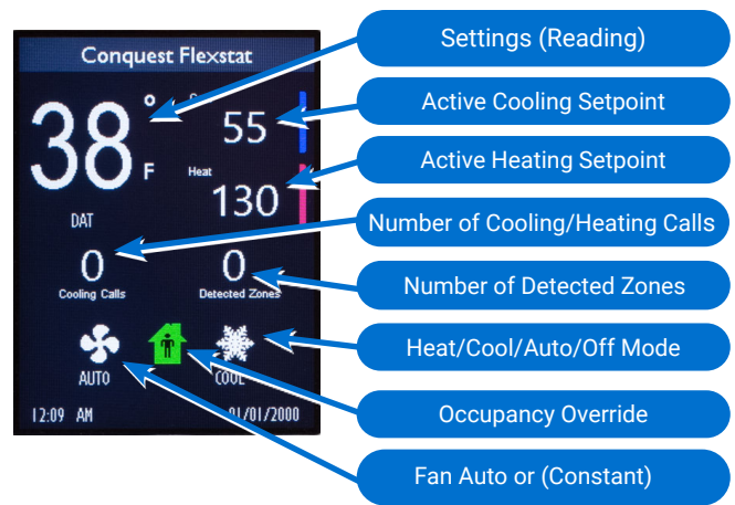
Illustration 13—Screen Menus Access (Default)
