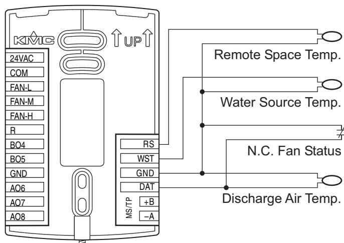
Illustration 4—FCU inputs
