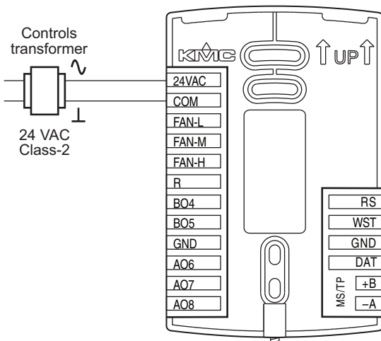
Illustration 6—Wiring for AppStat power
