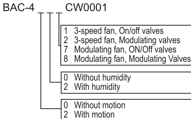
Illustration 1—Fan Coil Unit models
