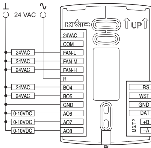
Illustration 5—FCU output terminals
