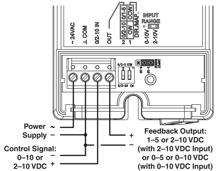
CK/745 Wiring (MEP-4002)
