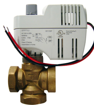
3-Way with 2-Position Fail-Safe Actuator
