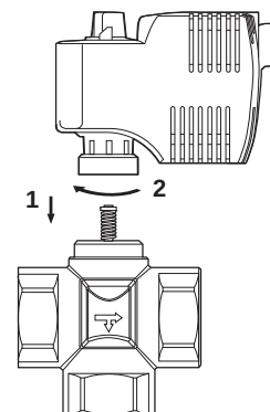
Mounting Actuator on Valve Body
