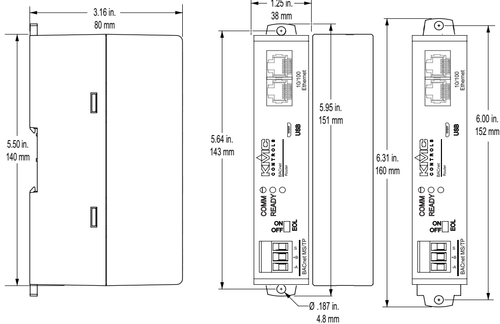
35 x 7.5 mm DIN rail mounting
