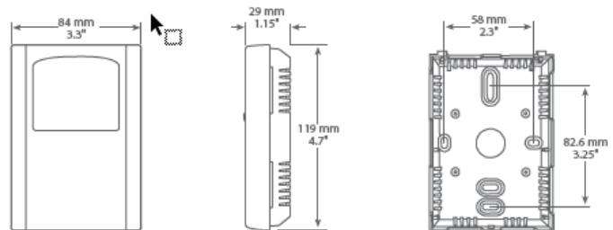
SAE-1011/1012 (Space)
