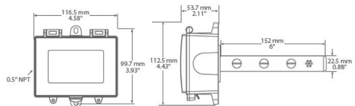
SAE-1062 (Duct)
