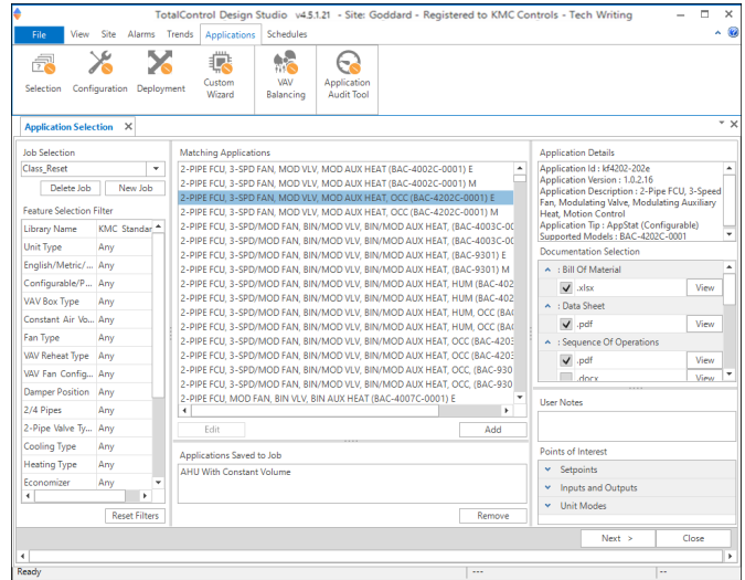
Application Wizard
