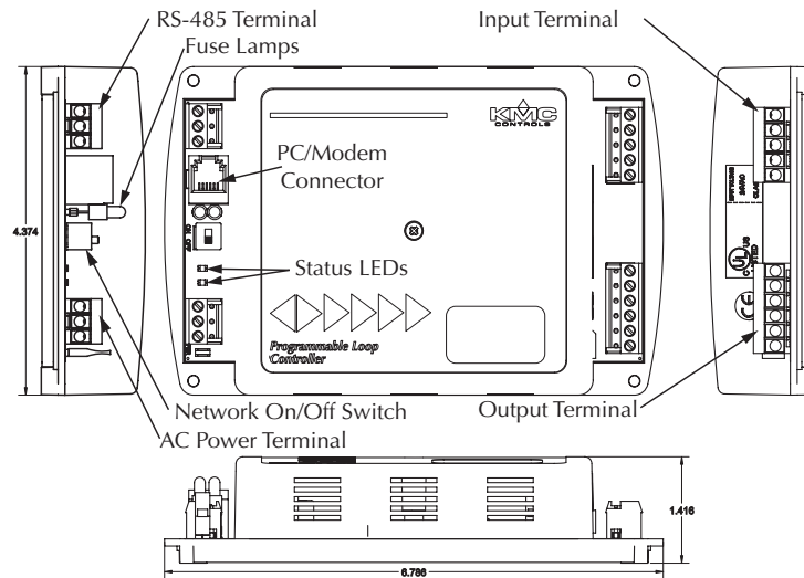
Illustration 1. Controller Components
