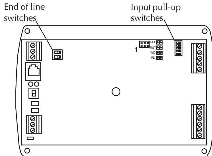
Illustration 4. Configuration Switch Locations
