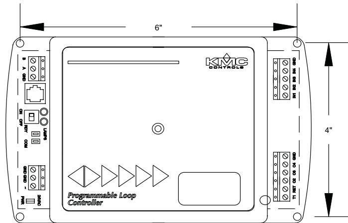
Illustration 3. Mounting Hole Locations
