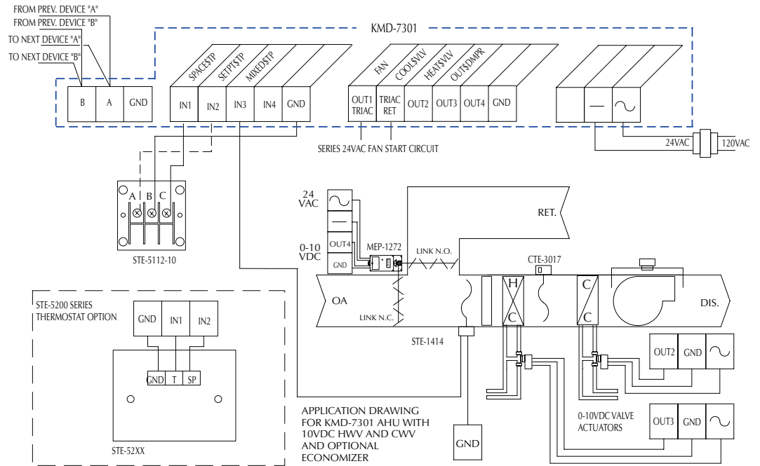
Illustration 6. Typical Controller Application Diagram
