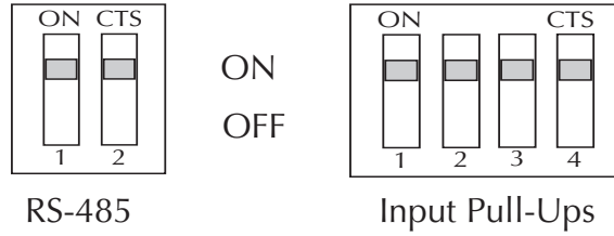
Illustration 5. Configuration Switches
