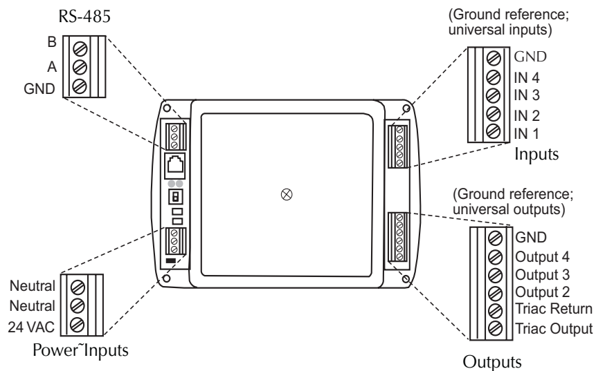
Illustration 2. Connector Detail
